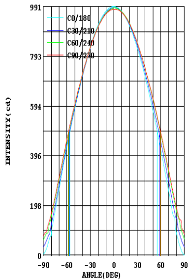
LUMINOUS INTENSITY DISTRIBUTION
