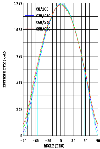
LUMINOUS INTENSITY DISTRIBUTION
